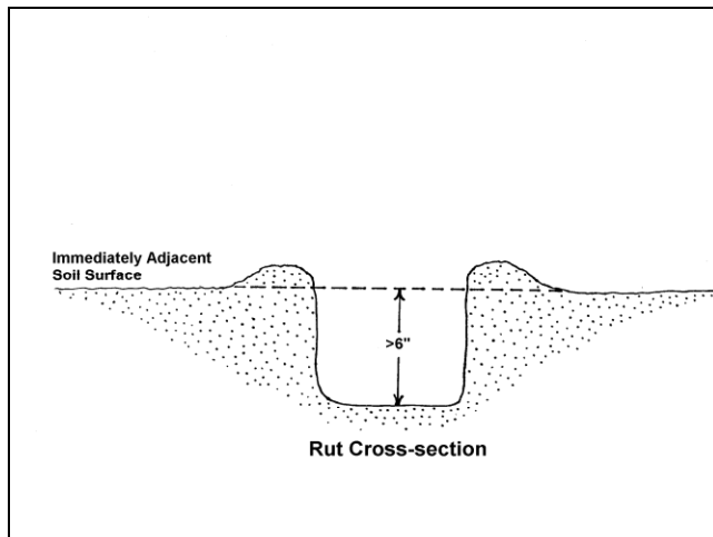
Rut Cross-Section
